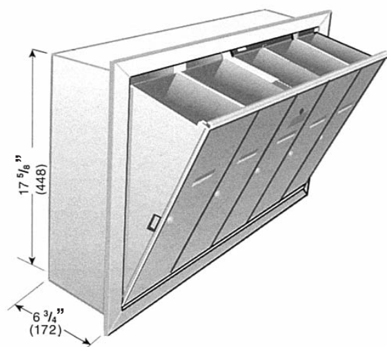
S-101 Recessed Wall Opening Sizes
