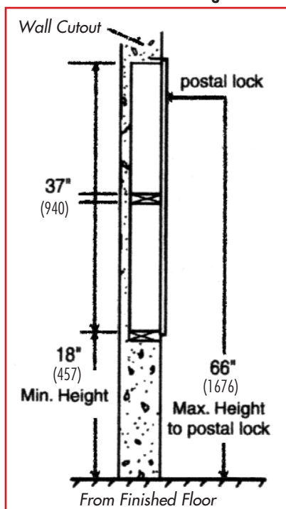
Double Row Installation Drawing
